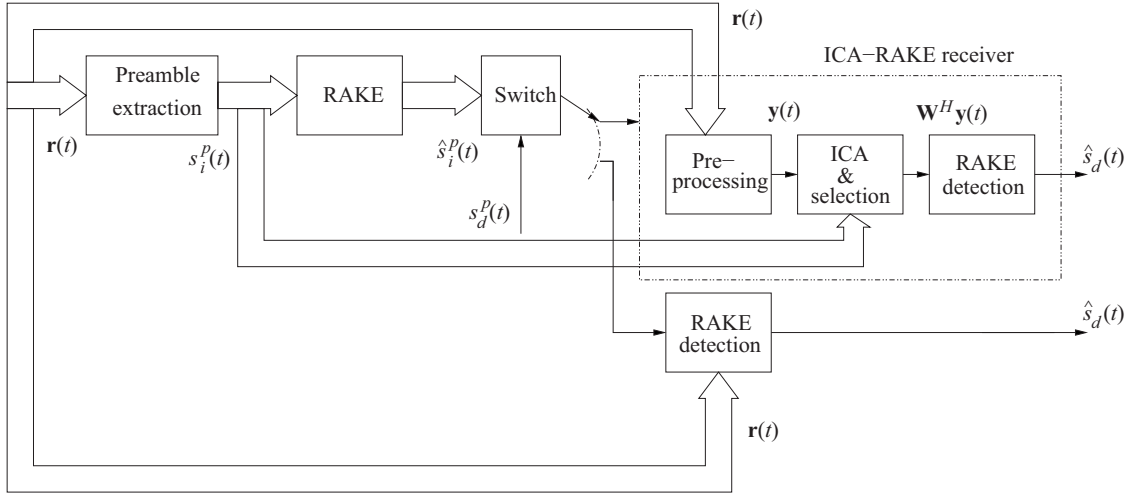
Fig. 1. ICA-RAKE pre-switching configuration. The preamble sequence s_d^p is used for switching between the two sections, and \mathbf{W} is the orthogonal separating matrix applied to the whitened version \mathbf{y}(t) of the received vector \mathbf{r}(t) .
